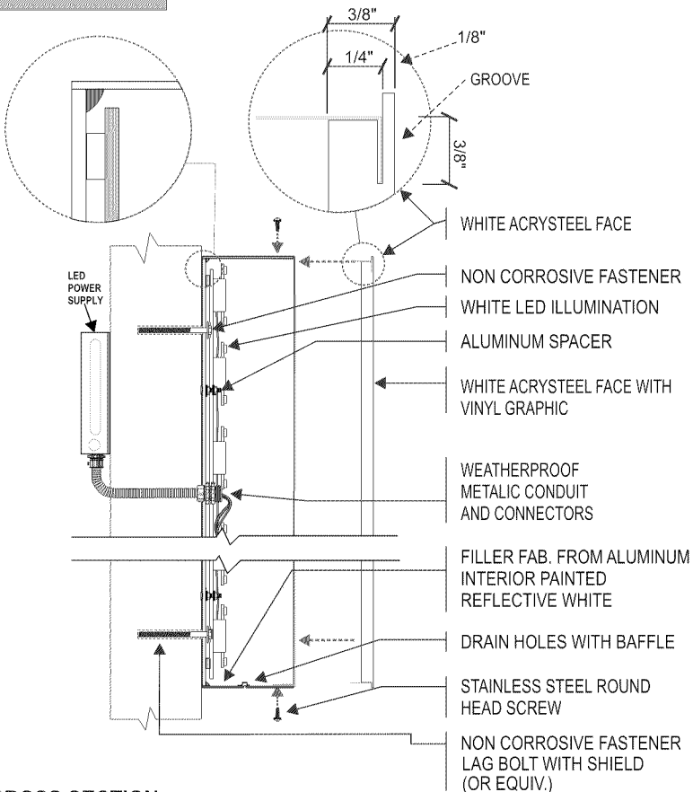
CROSS SECTION
