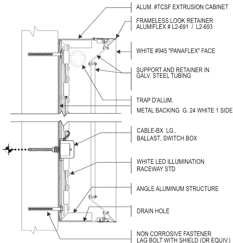
CROSS SECTION
