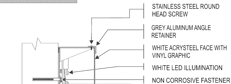
CROSS SECTION
