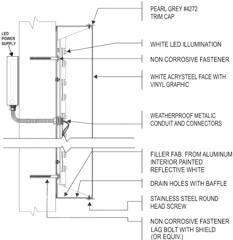
CROSS SECTION
