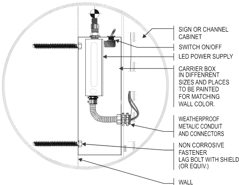
DETAIL - CROSS SECTION
