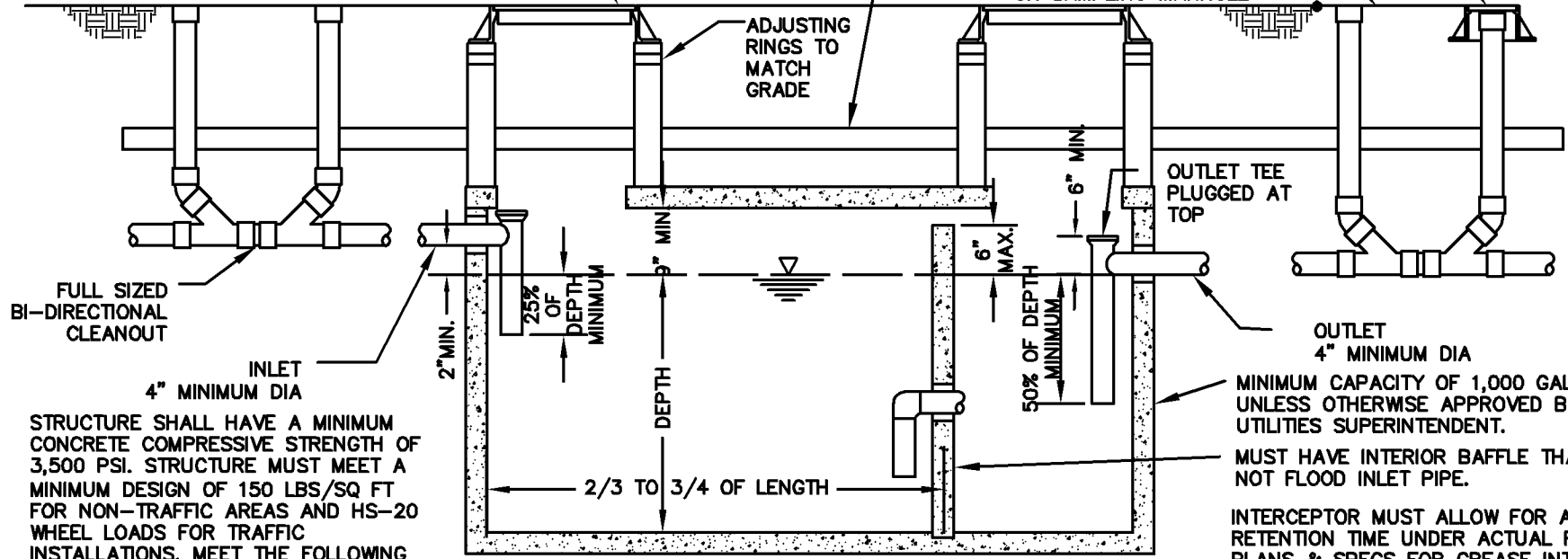
PROFILE VIEW
