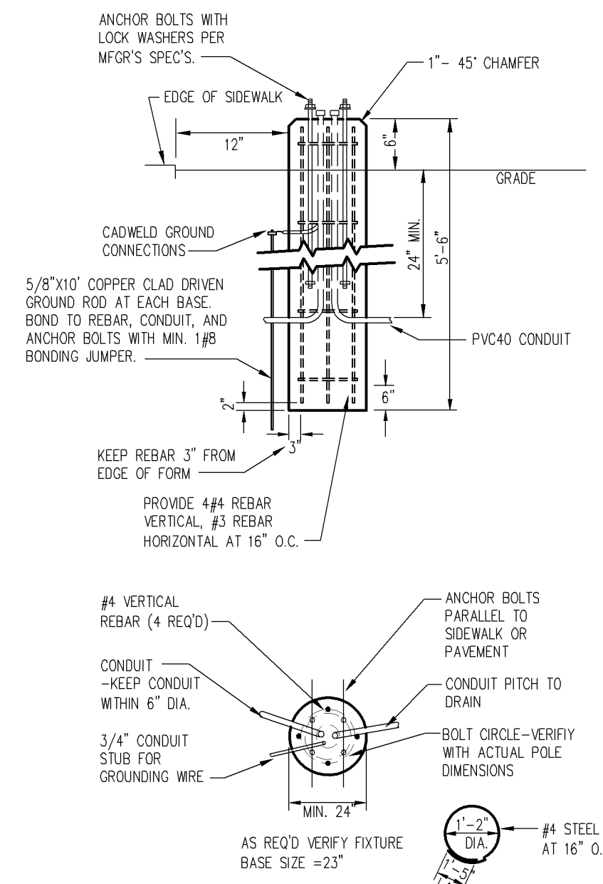
2 POLE BASE DETAIL NOT TO SCALE
