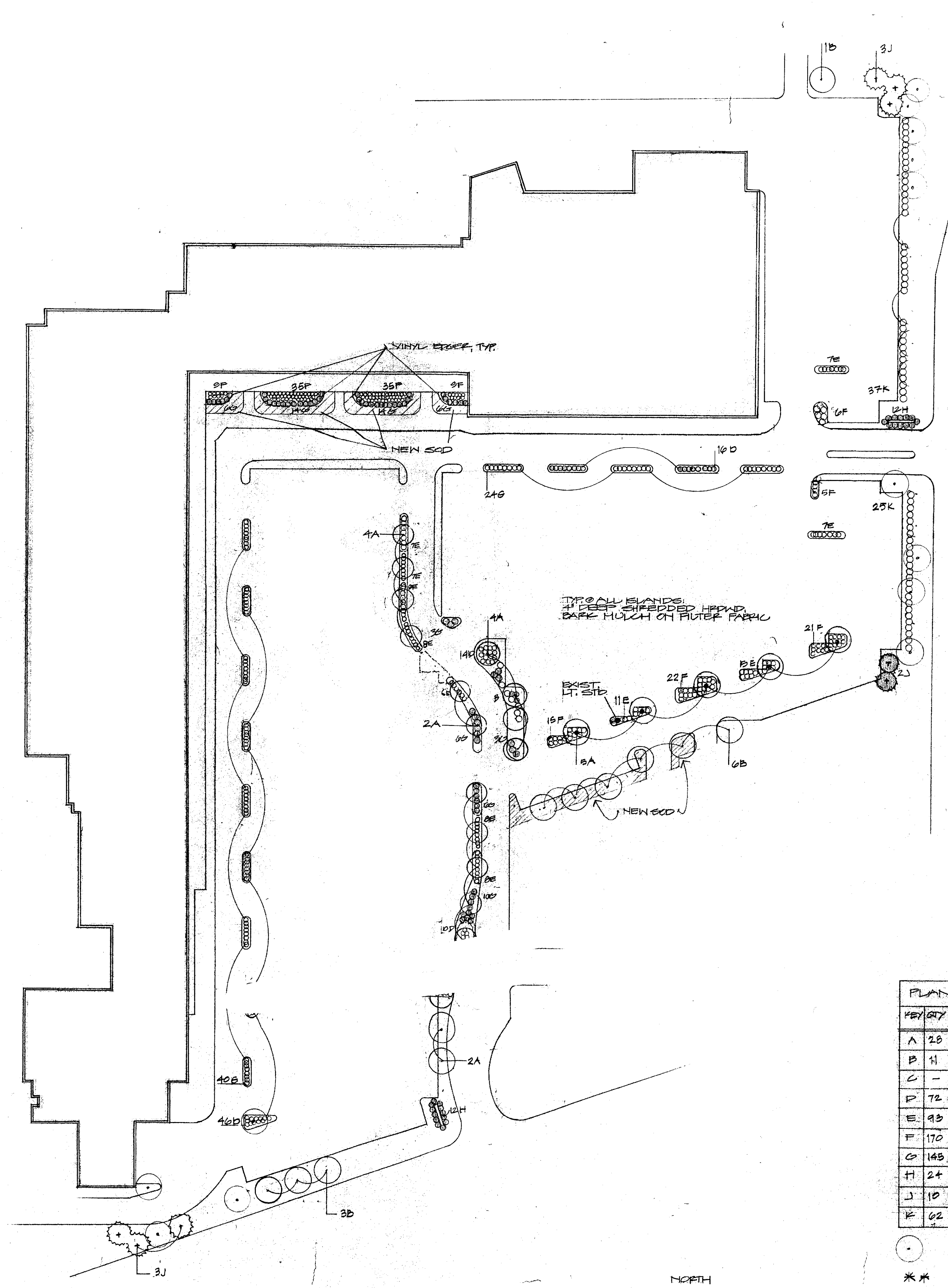
FENCED LANDSCAPE PLAN SCALE: 1"=50'
