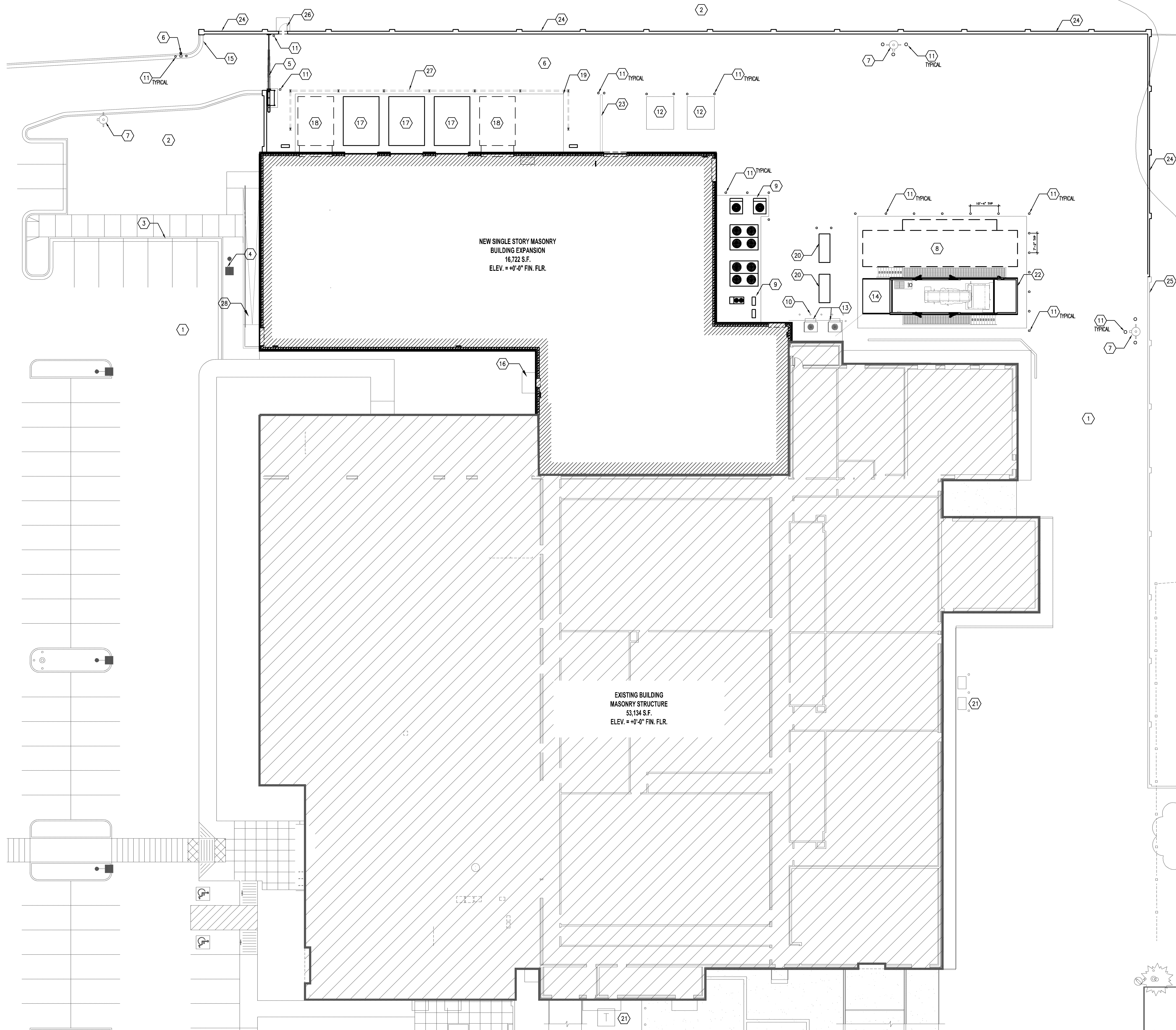
1 ARCHITECTURAL ENLARGE SITE PLAN A101 SCALE: 1/16" = 1'-0"
