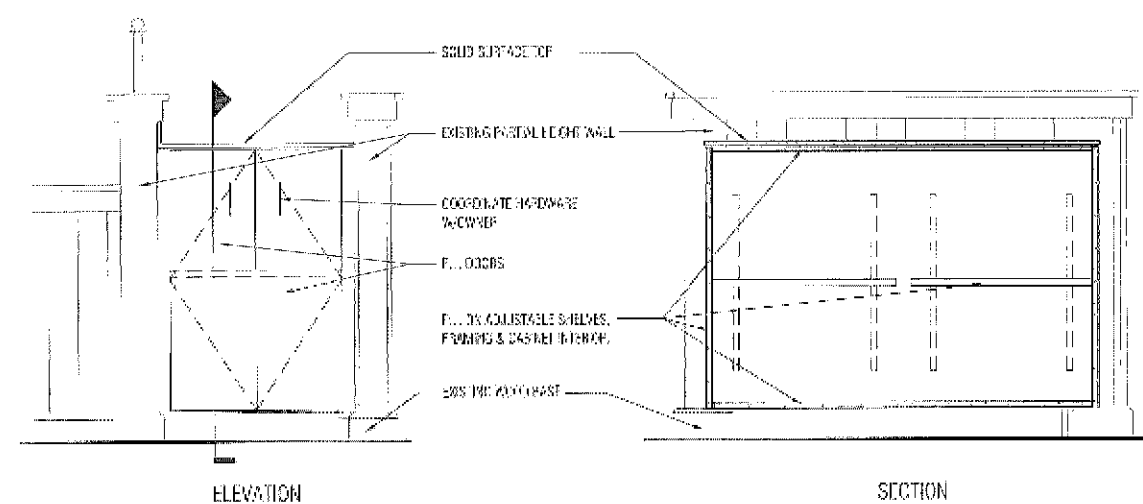
5 HOSTESS STAND DETAILS (TYP) SCALE: 1/2"=1'-0"
