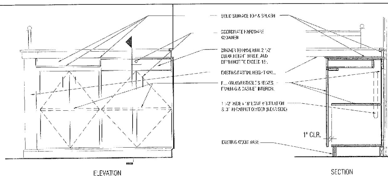
9 SERVER STAND DETAILS (TYP) SCALE: 1/2"=1'-0"
