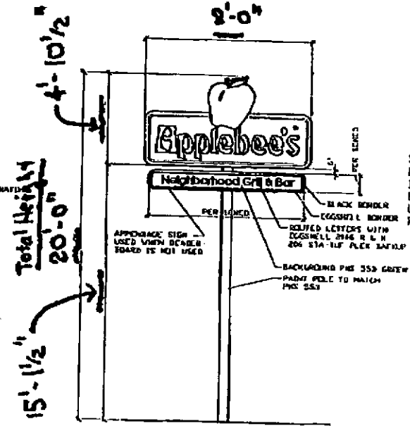
TYP. POLE SIGN W/O READERBOARD 16' WIDE UNIT SHOWN NO SCALE
