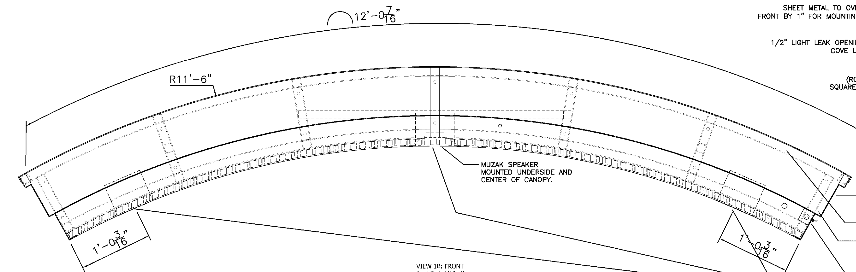
VIEW 1B: FRONT SCALE: 1-1/2"=1'
