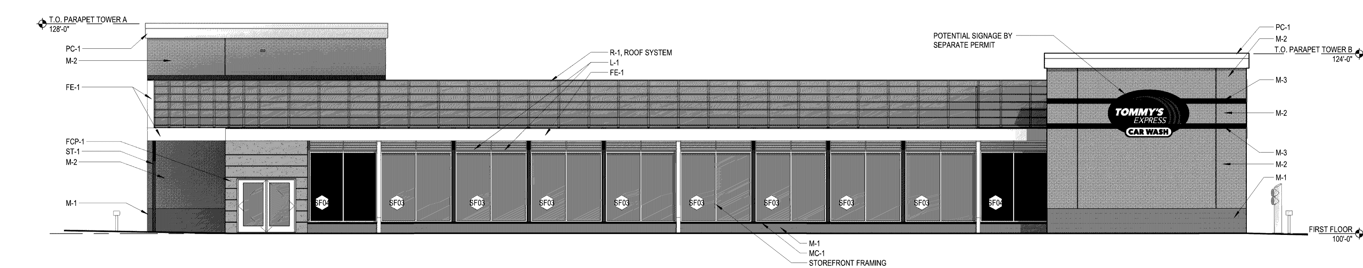
4 BACK ELEVATION A101 1/8" = 1'-0"
