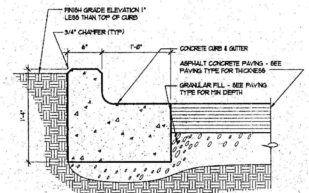
7 CONCRETE CURB DETAIL @ PAVEMENT EDGE A1.0
