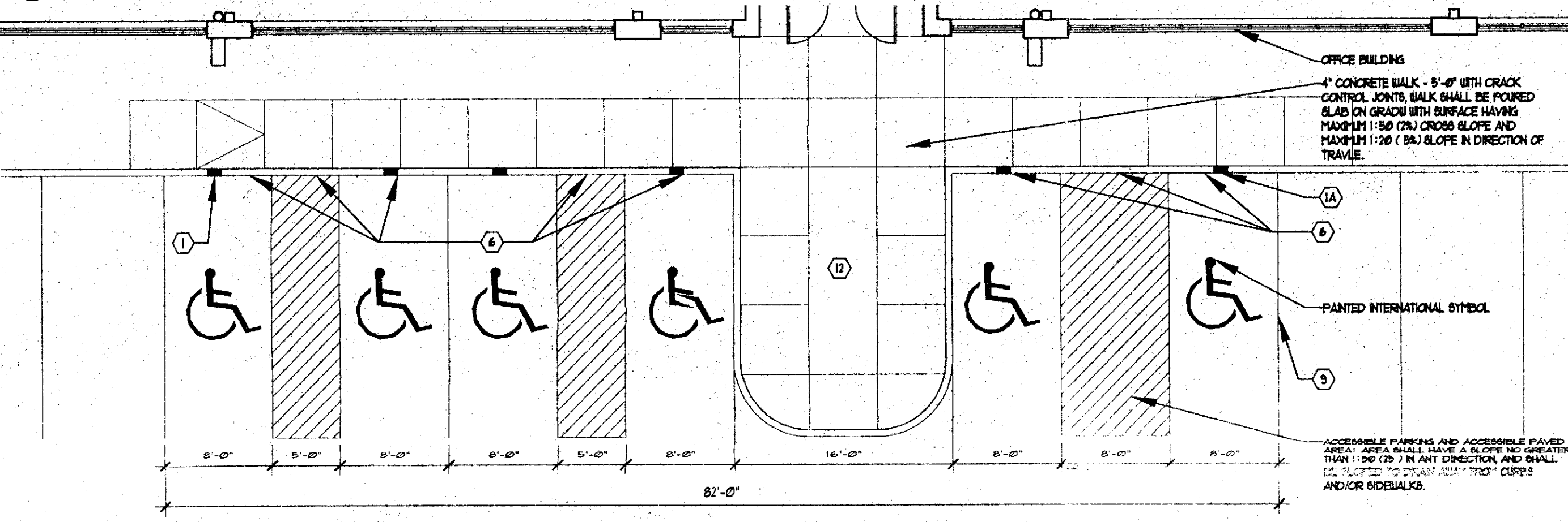
5 ACCESSIBLE PARKING LAYOUT A1.0
