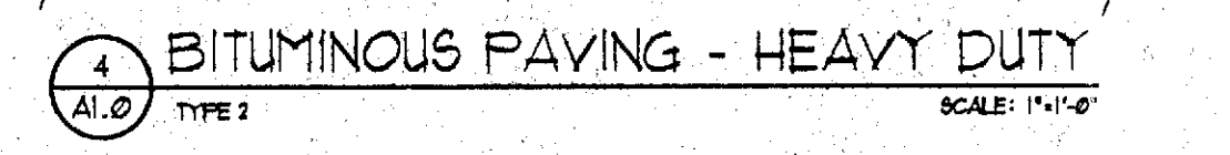
4 BITUMINOUS PAVING - HEAVY DUTY A1.0 TYPE 2
