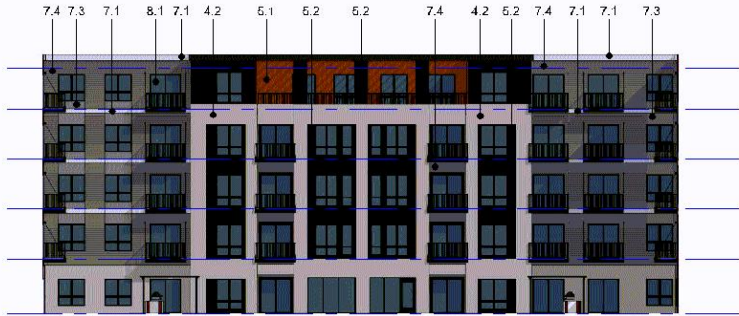
1 South - Plaza 3/64" = 1'-0"
