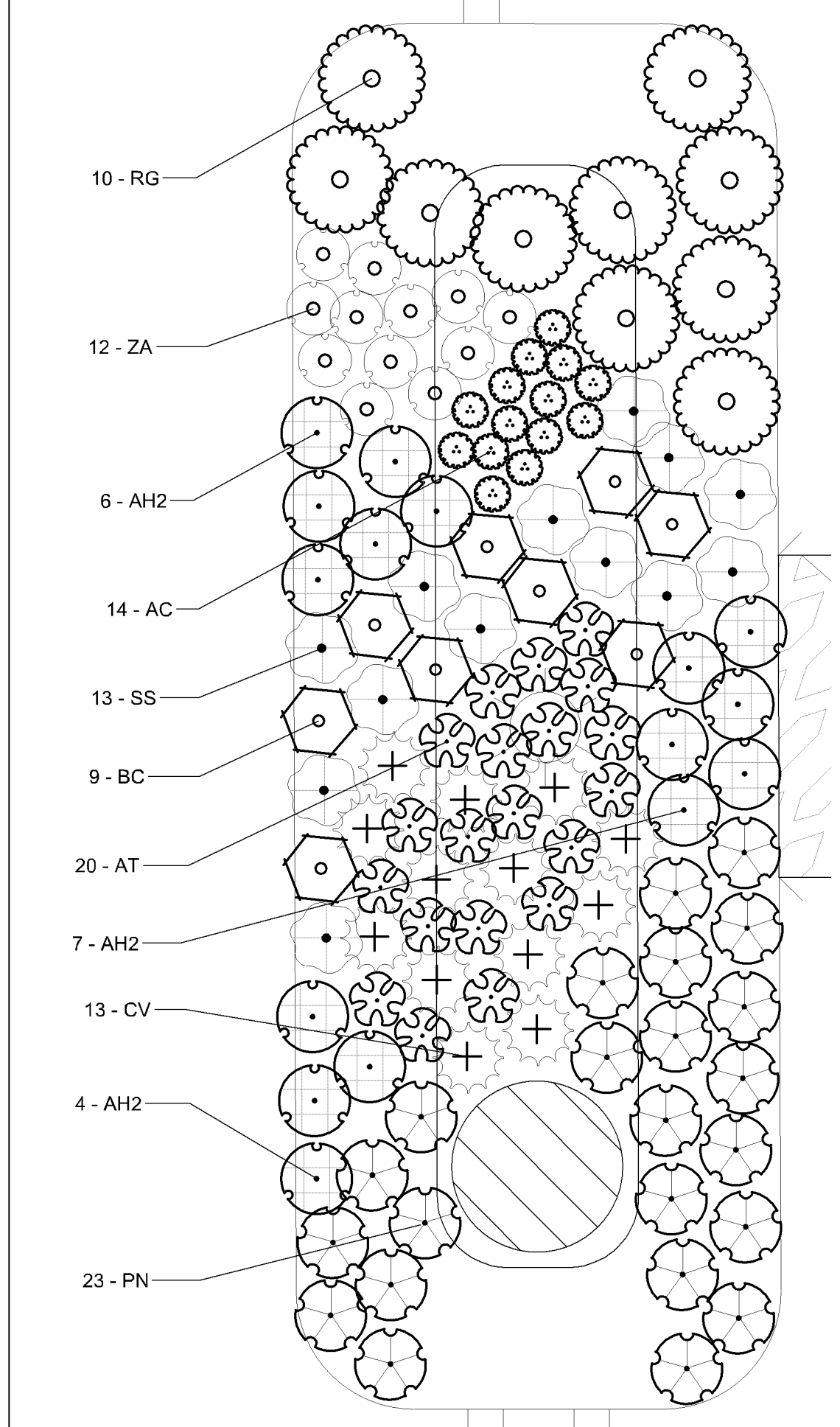
02 ENLARGEMENT C Scale: 1/4" = 1' - 0"
