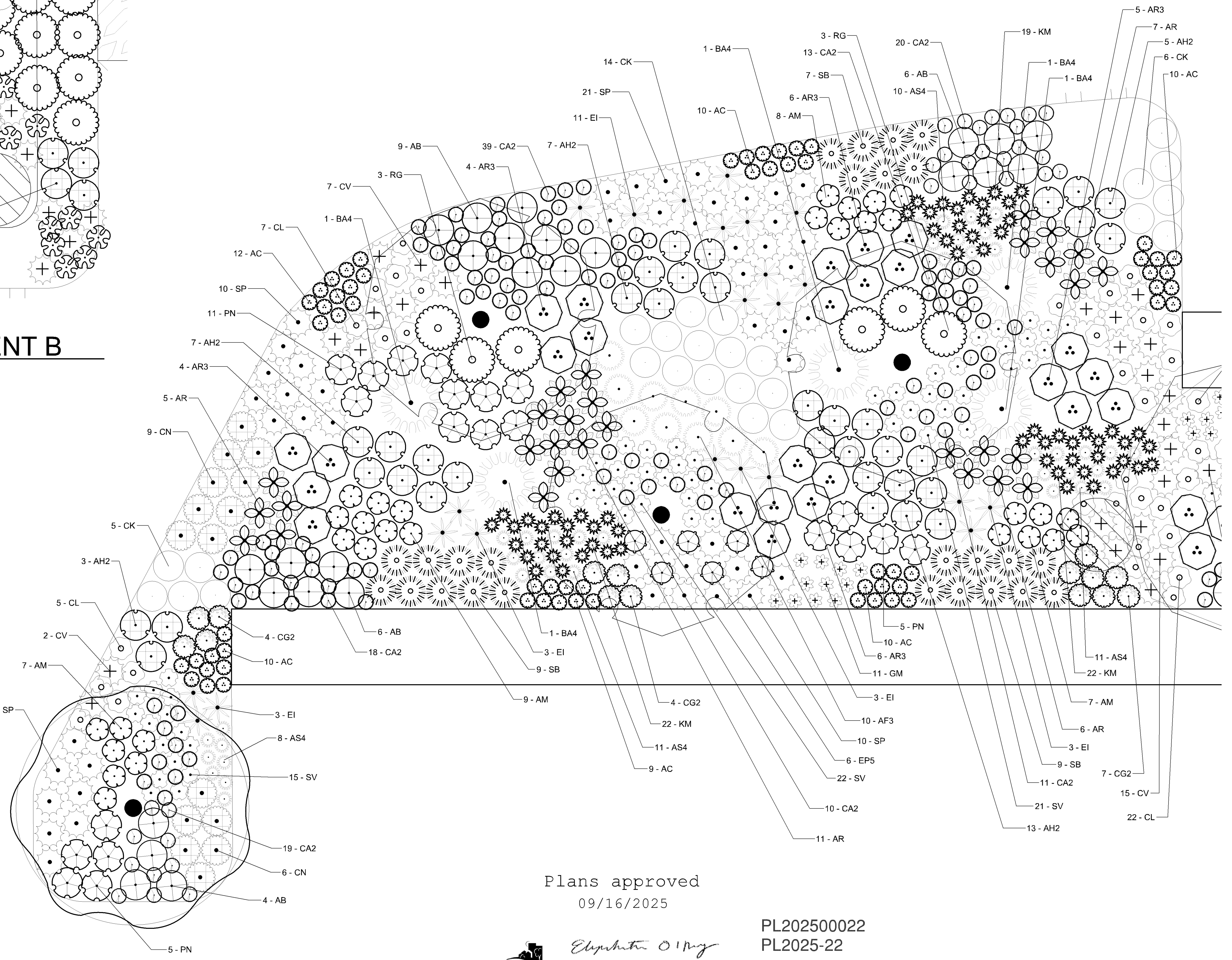
01 ENLARGEMENT 01 Scale: 1/4" = 1' - 0"
