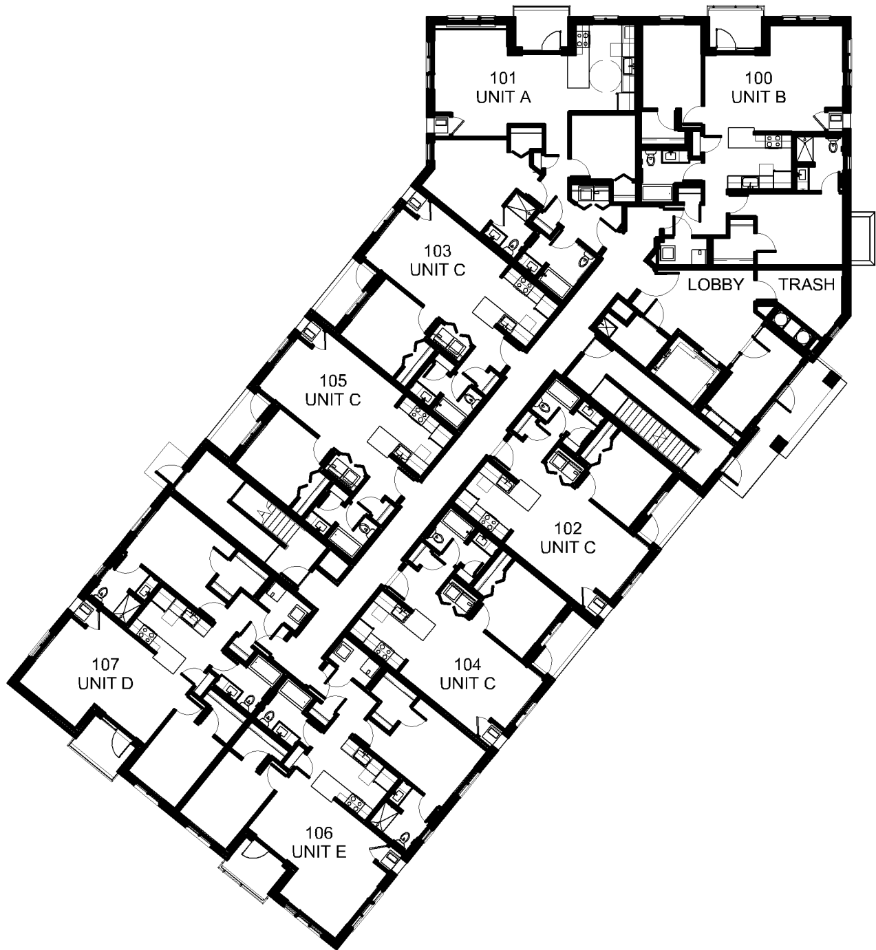
1 FIRST FLOOR PLAN 1" = 20'-0"
