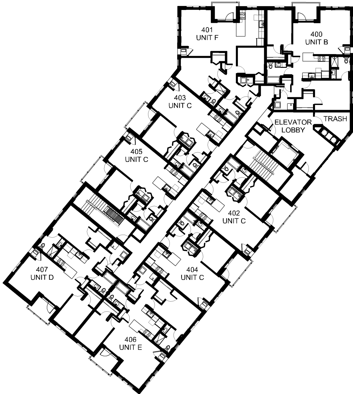
1 FOURTH FLOOR PLAN 1" = 20'-0"
