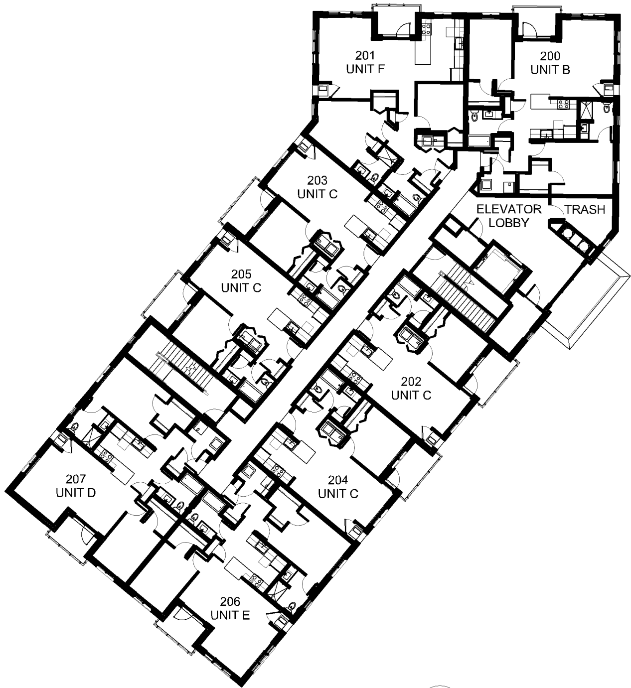
1 SECOND FLOOR PLAN 1" = 20'-0"
