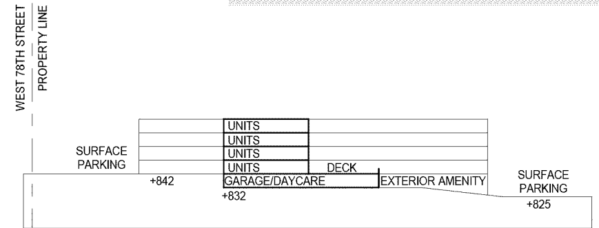
Section Cut A
