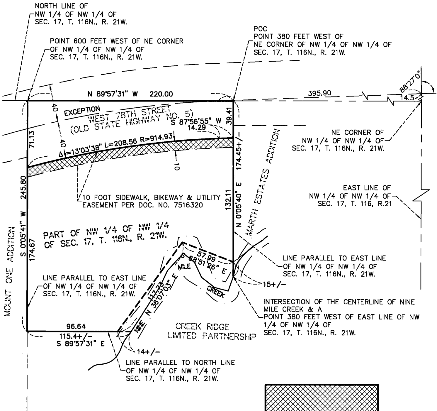
VACATED 10 FOOT SIDEWALK, BIKEWAY & UTILITY EASEMENT
