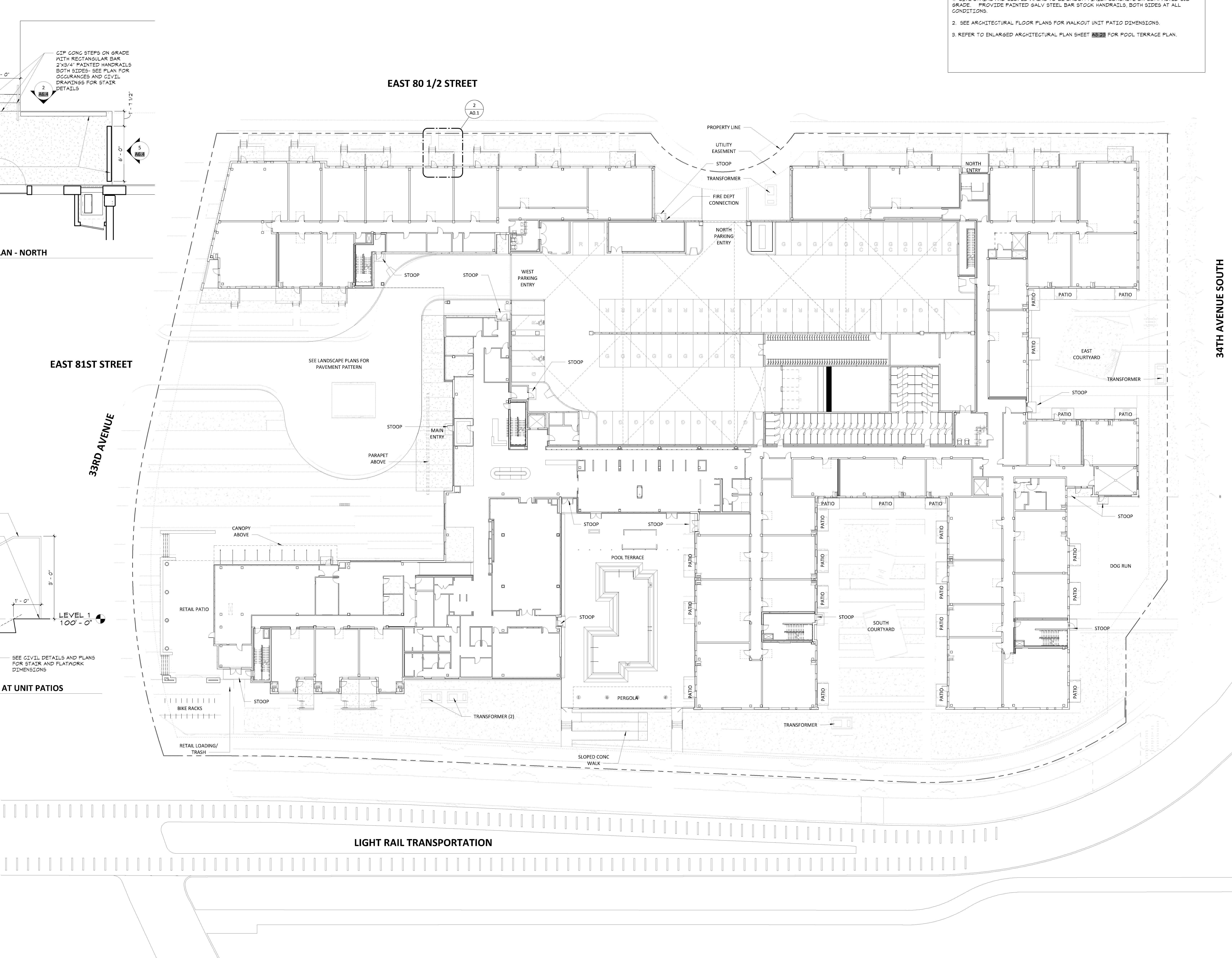
1 ARCHITECTURAL SITE PLAN A0.1 1" = 20'-0"
