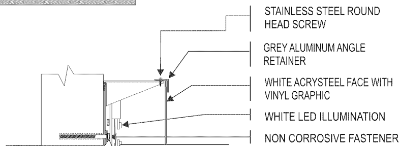
CROSS SECTION
