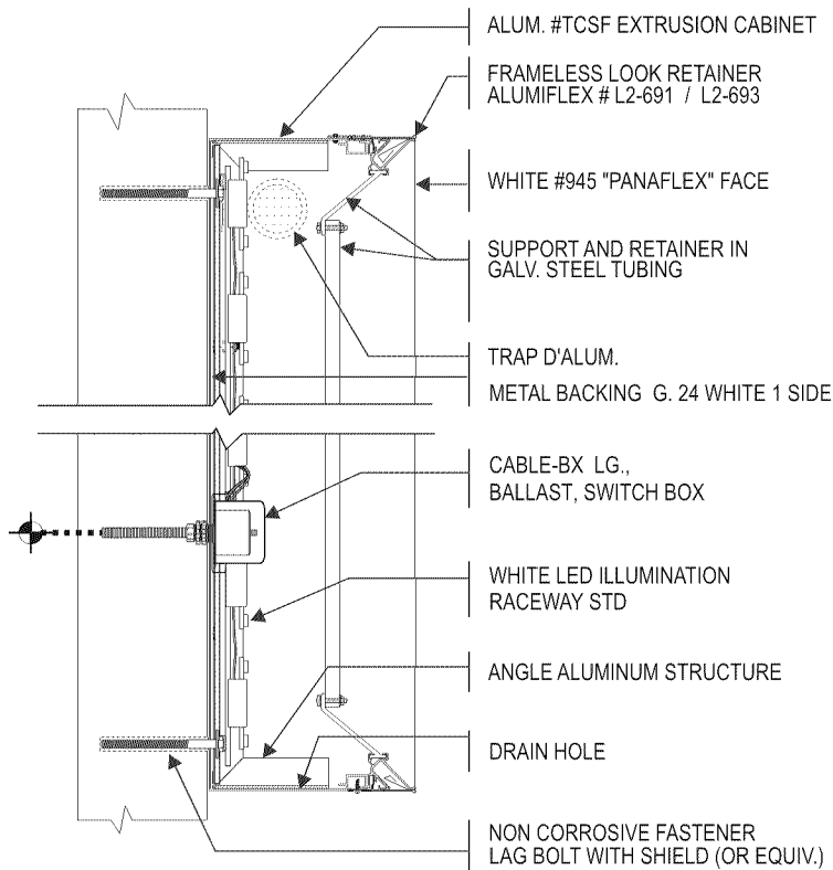
CROSS SECTION
