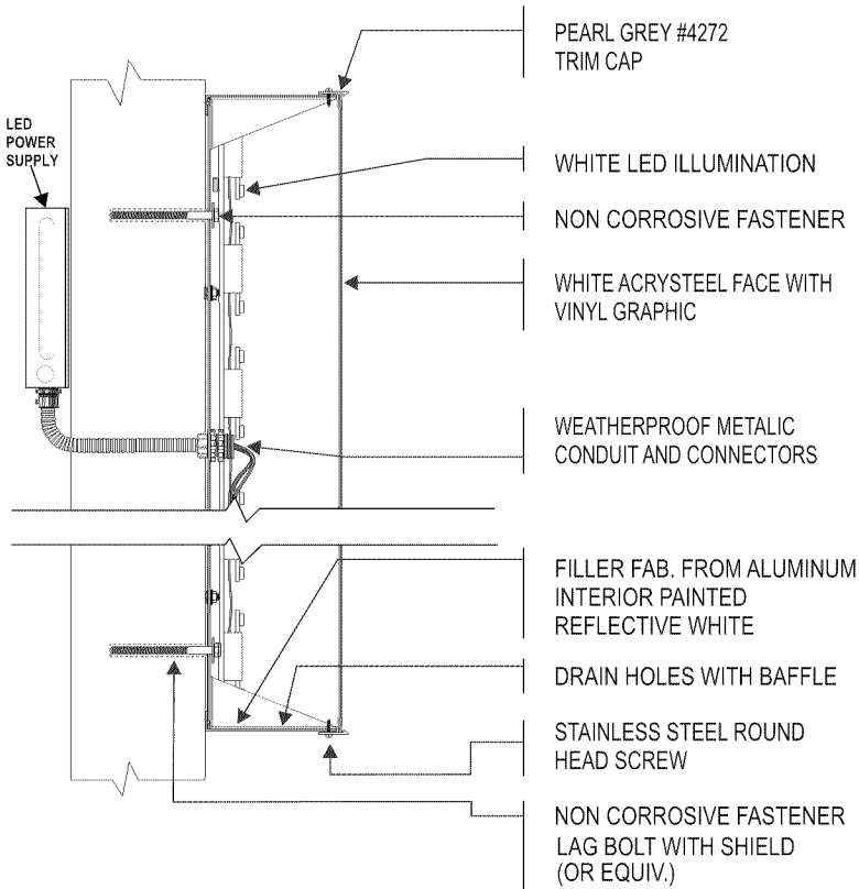
CROSS SECTION
