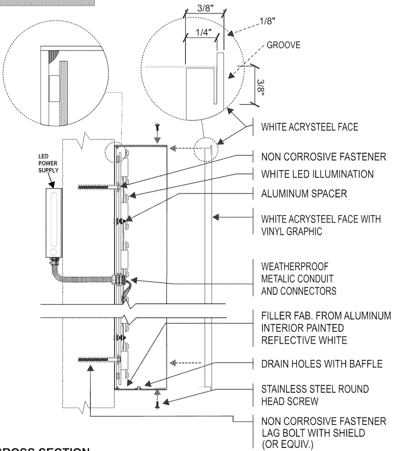
CROSS SECTION
