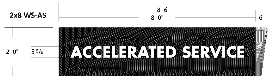
2x8 Acura S/F Illuminated Wall Sign - Routed Out and Pushed Through
