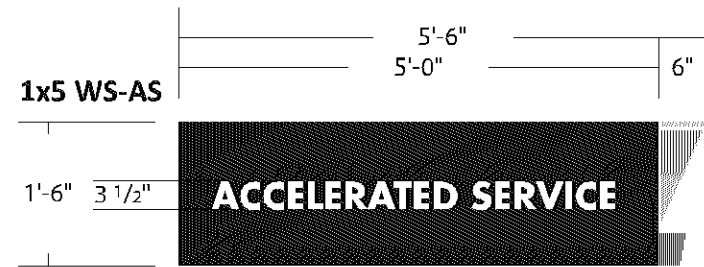
1x5 Acura S/F Illuminated Wall Sign - Routed Out and Pushed Through
