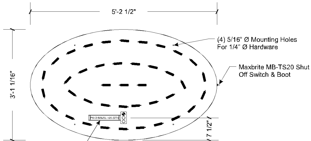
LED LAYOUT SCALE: 3/4" = 1'-0"
