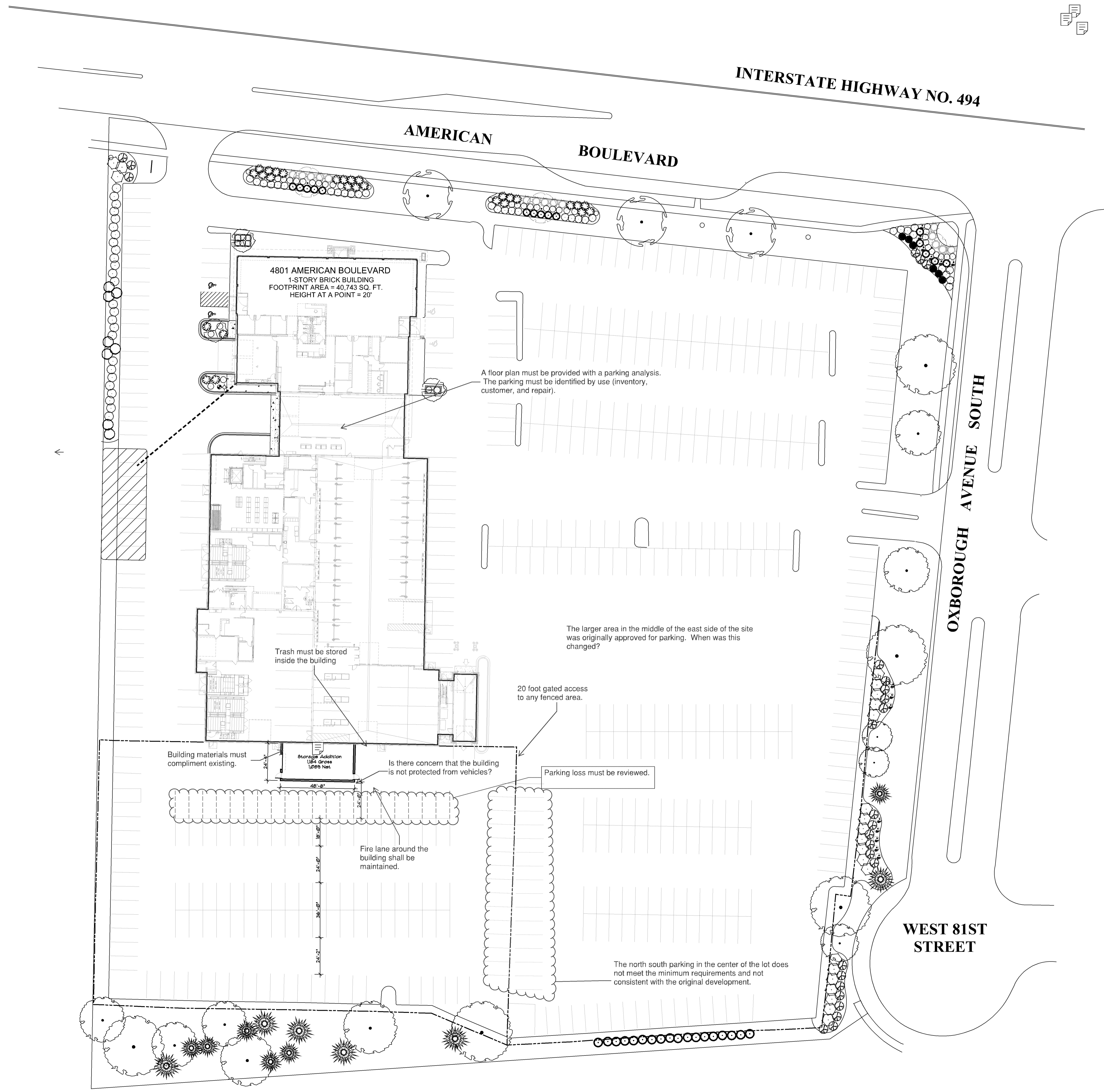
A3 Site Plan 1"=30'-0"
