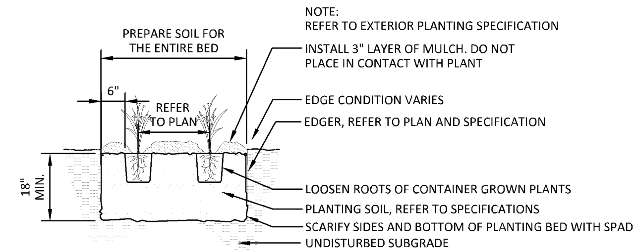
3 PERENNIAL PLANTING DETAIL 1/2" = 1'-0" P-03
