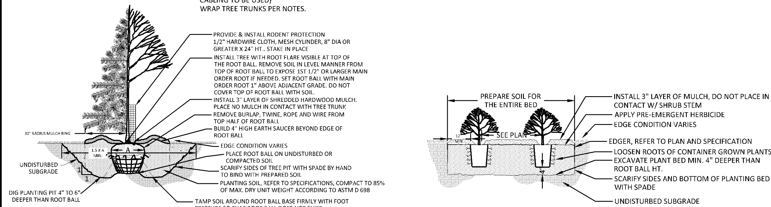
1 L1.02 1/4" = 1'-0"
