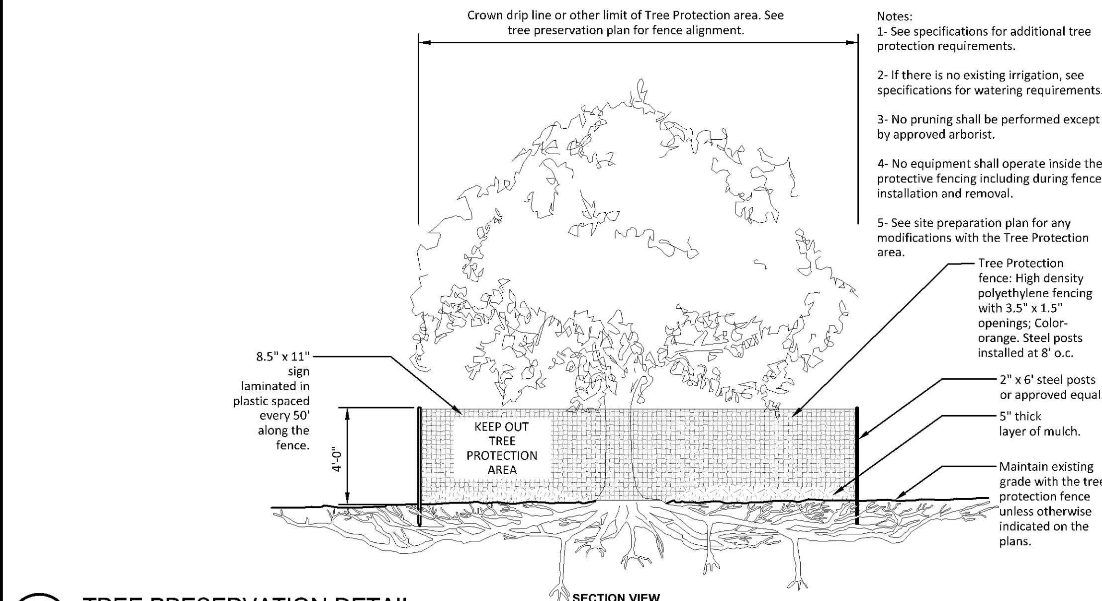
5 L1.02 1/4" = 1'-0"
