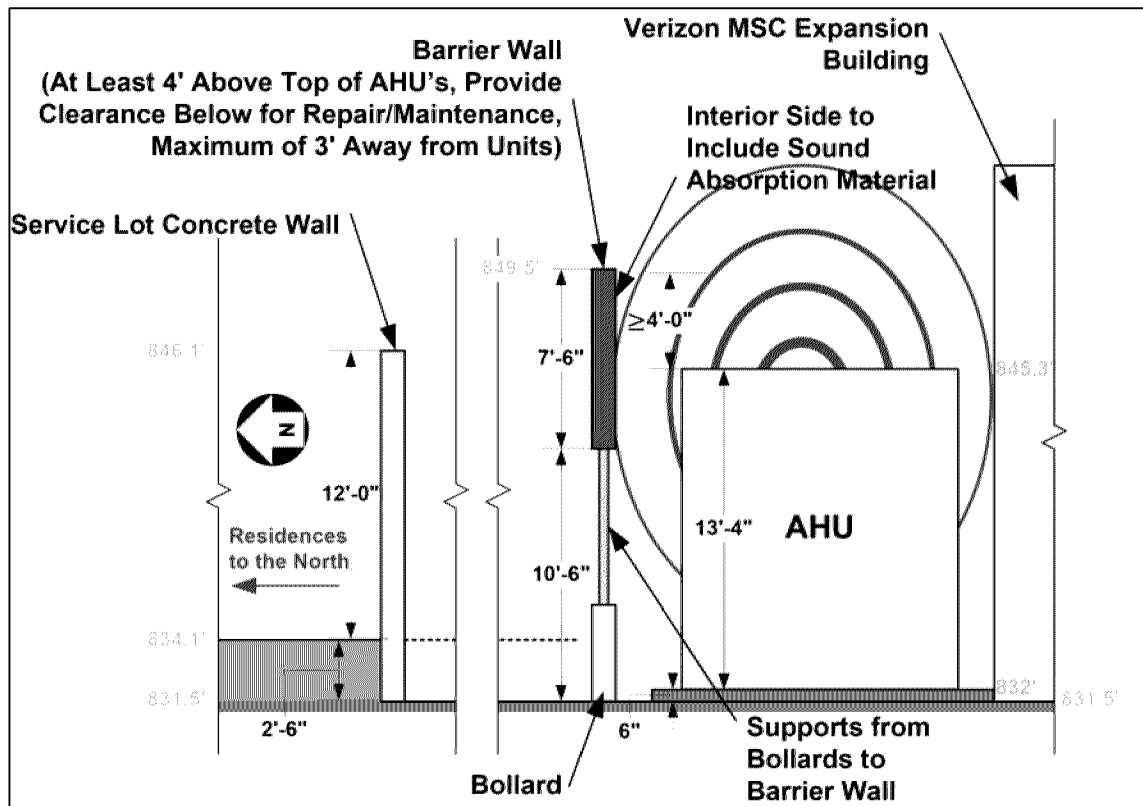
Figure 3 – Elevation sketch of the proposed AHU noise control barrier wall.
