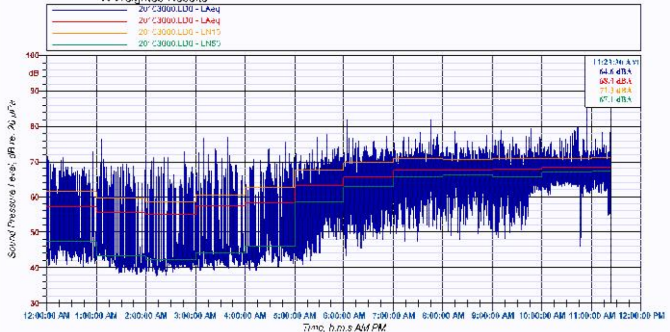
Noise Monitoring Measured Hourly LAeq Data
