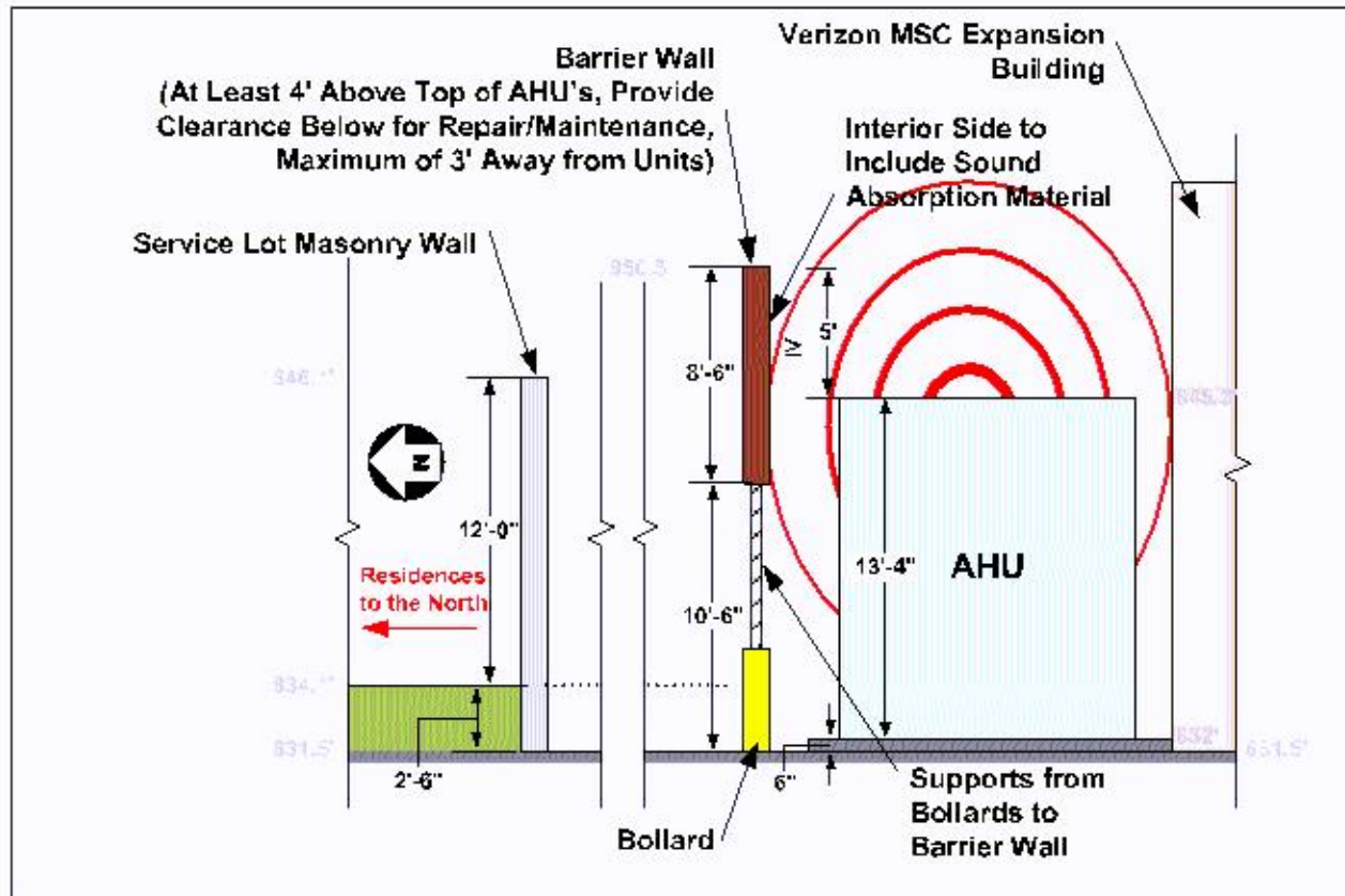
Figure 4 - Elevation sketch of the proposed AHU noise control barrier wall.
