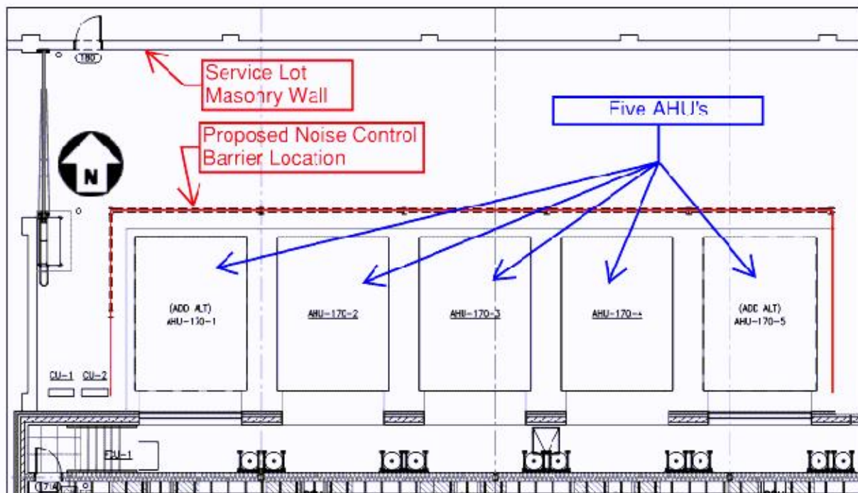
Figure 5 - Partial plan view showing the layout and location of the proposed barrier wall.
