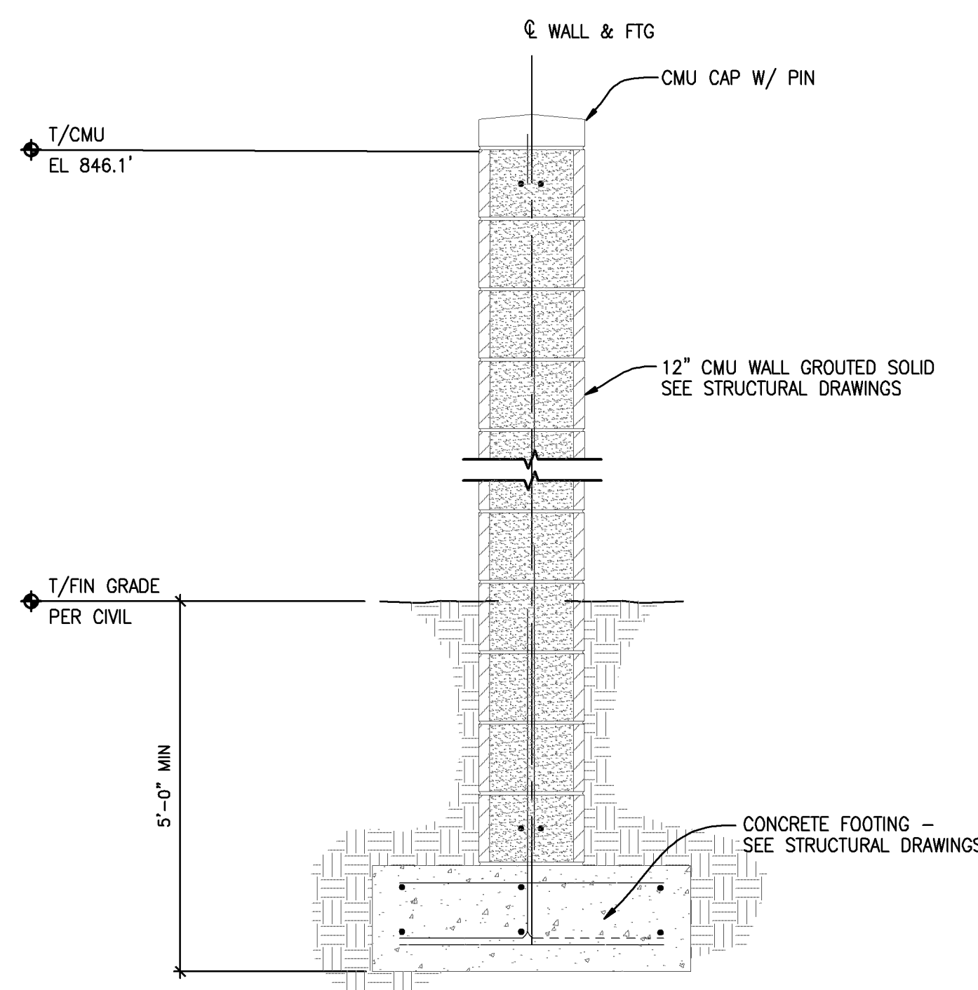
TALL CMU SCREEN WALL
