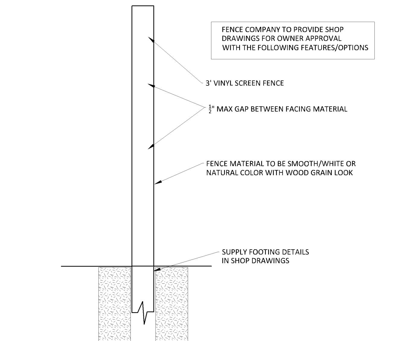
6 3'-0" SCREEN FENCE L1.04 1/8" = 1'-0" P-VI-02
