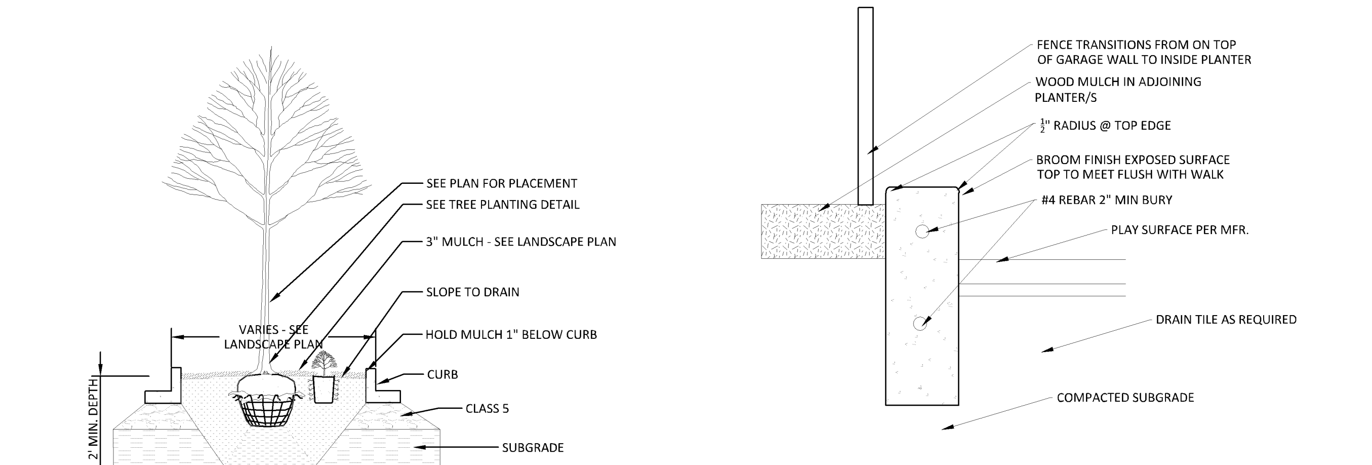
5 PARKING LOT ISLAND L1.04 1/4" = 1'-0" P-07
