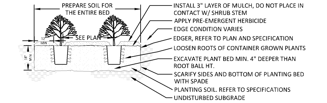
2 SHRUB PLANTING DETAIL L1.04 3/8" = 1'-0" P-02
