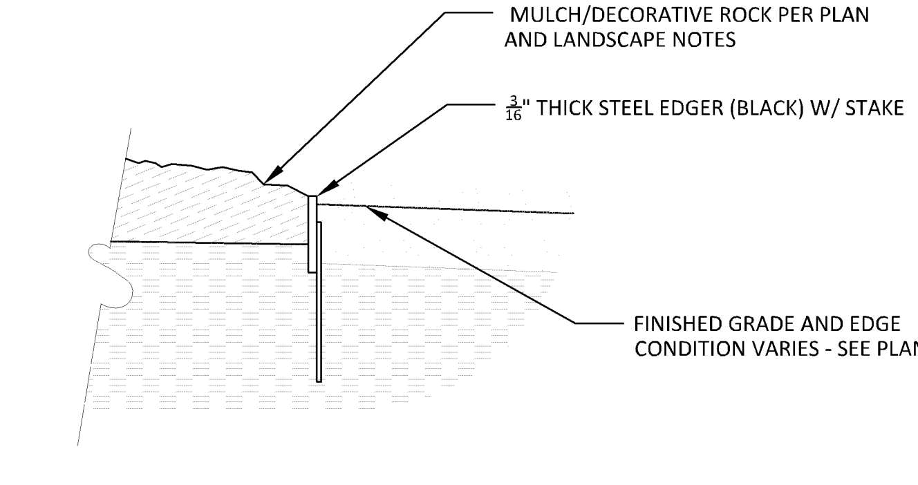
4 STEEL EDGER L1.04 1 1/2" = 1'-0" P-06
