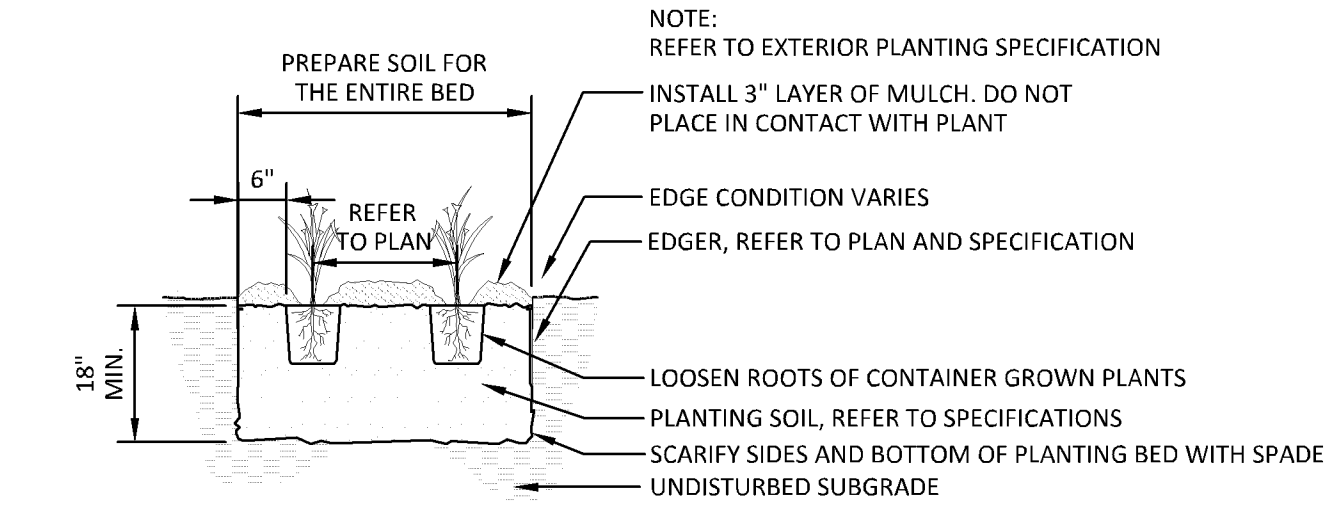
3 PERENNIAL PLANTING DETAIL L1.04 1/2" = 1'-0" P-03
