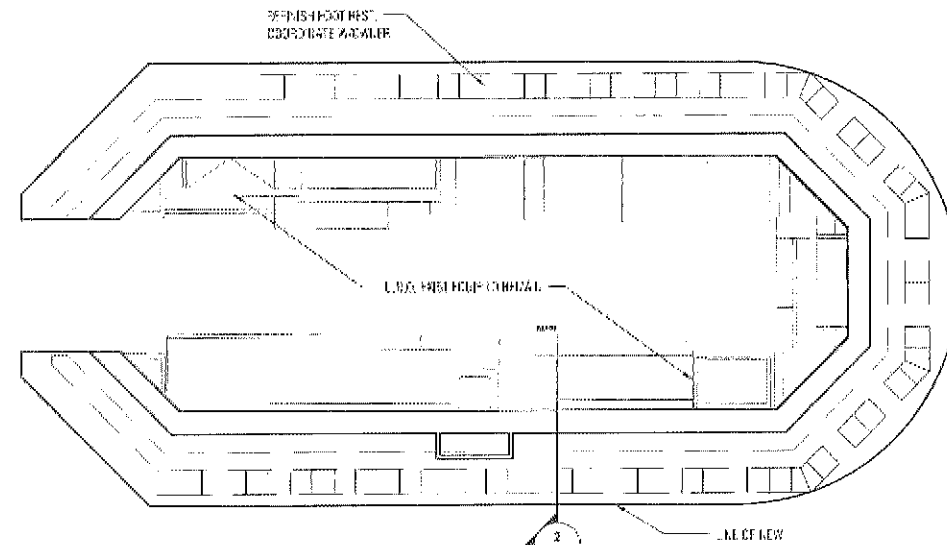
1 PROPOSED BAR PLAN SCALE: 1/2"=1'-0"
