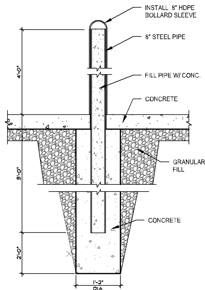
F15 BOLLARD DETAIL NOT TO SCALE
