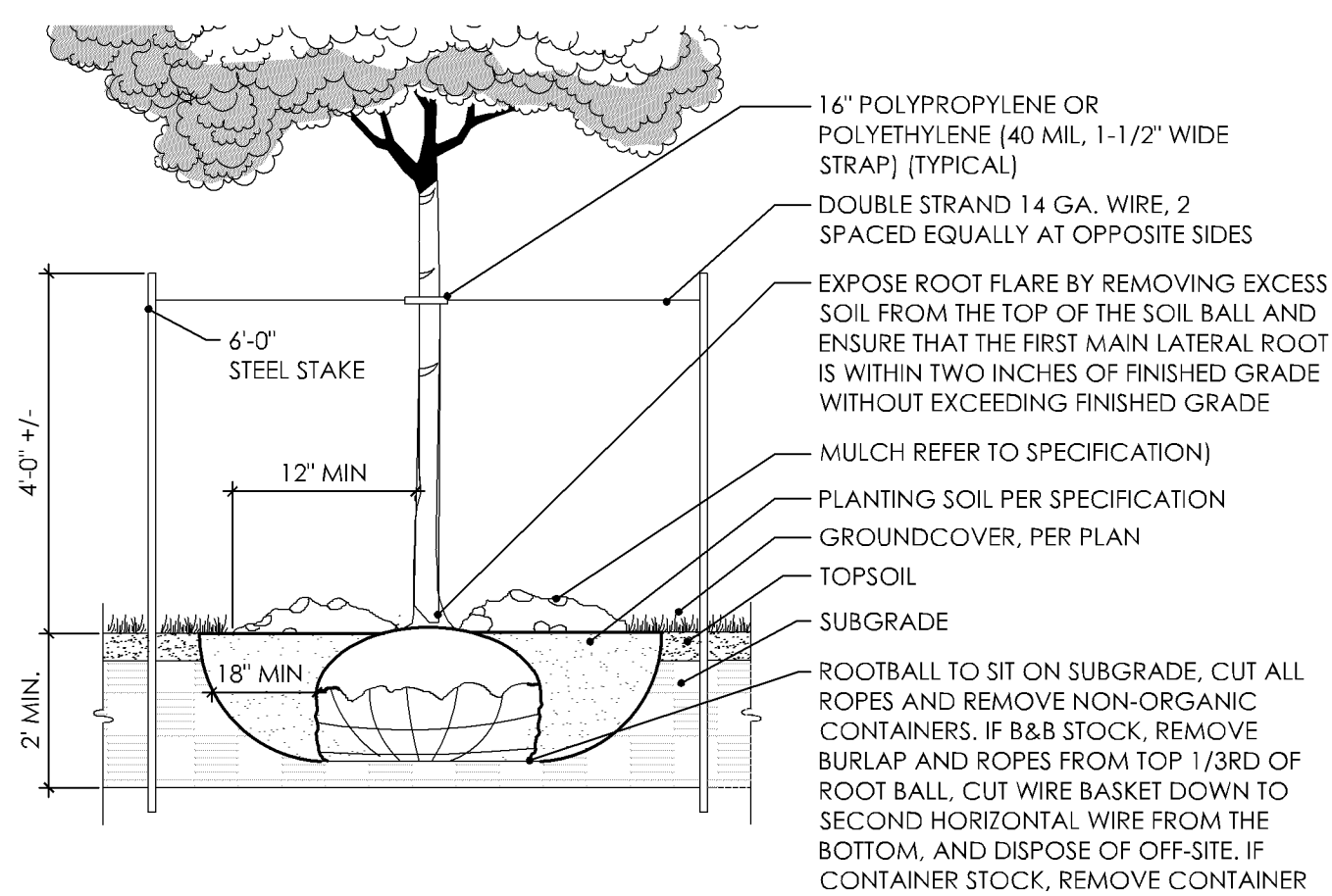
2 deciduous tree planting typ. scale: NTS
