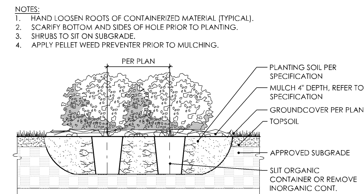
3 shrub planting typ. scale: NTS
