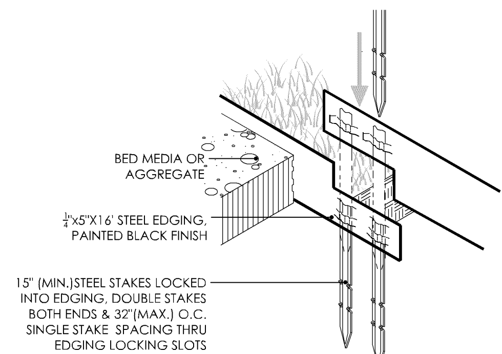
5 landscape edging typ. scale: NTS
