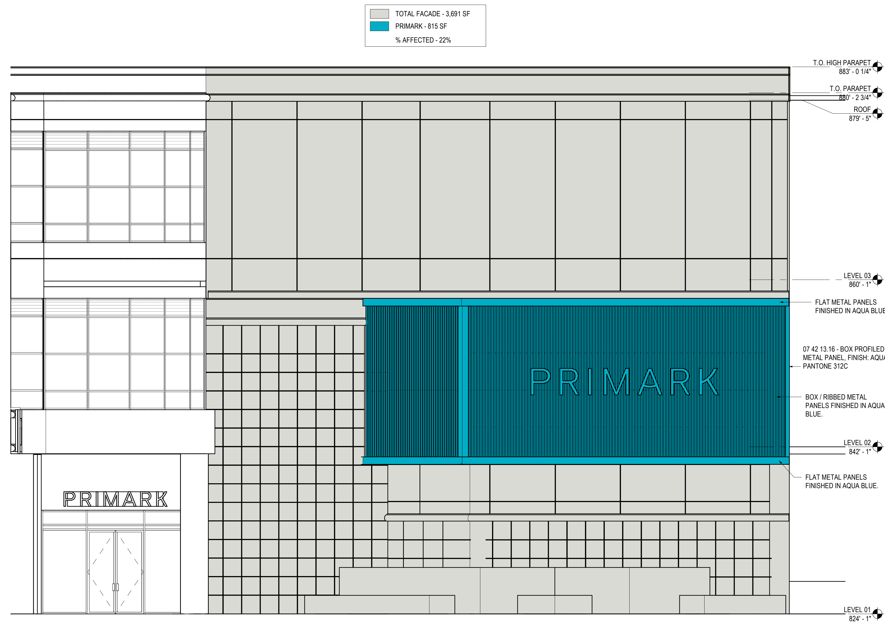
03 FACADE EAST - DIAGRAMATIC SCALE: 3/16" = 1'-0"
