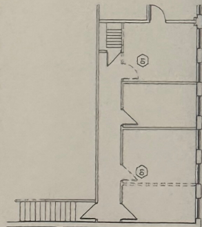
3 MEZZANINE DEMO PLAN 1/8"=1'-0"
